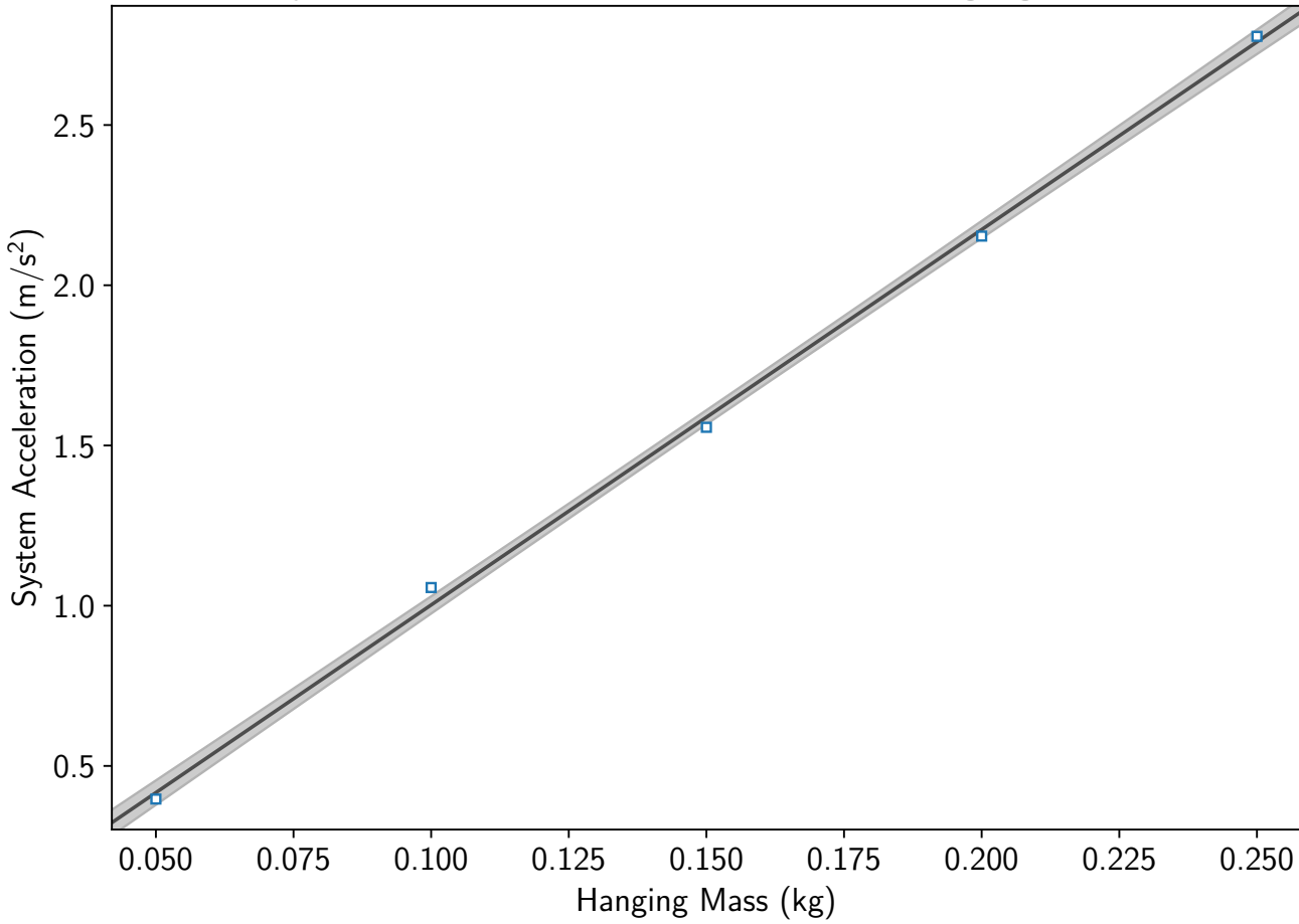
System Acceleration vs Different Hanging Mass
