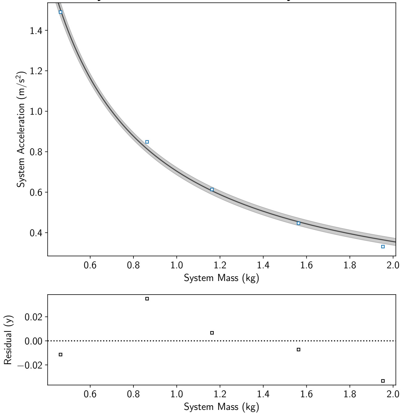
System Acceleration vs Different System Mass
