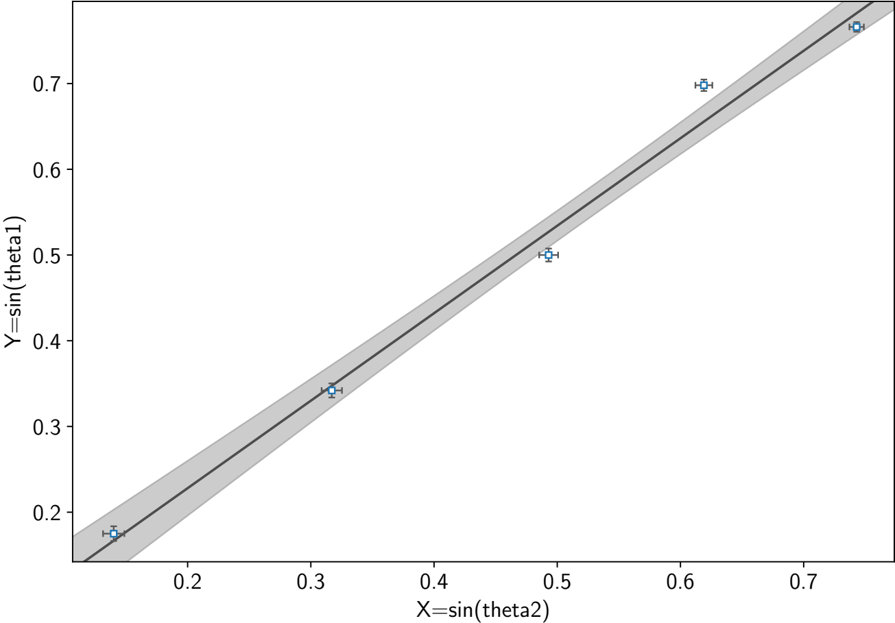
sin(theta1) vs sin(theta2)
