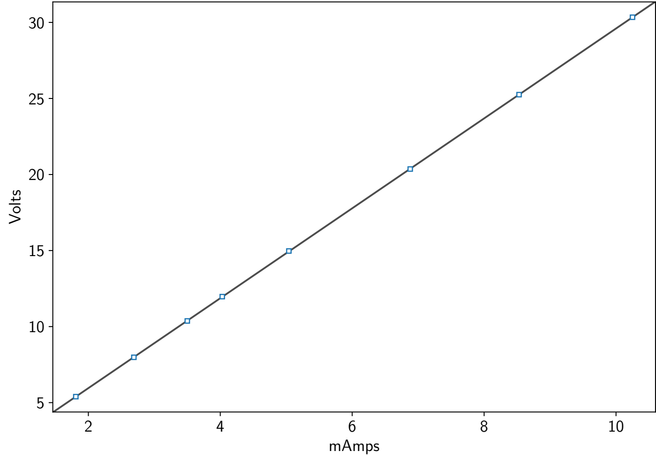
Amps vs Volts graph
