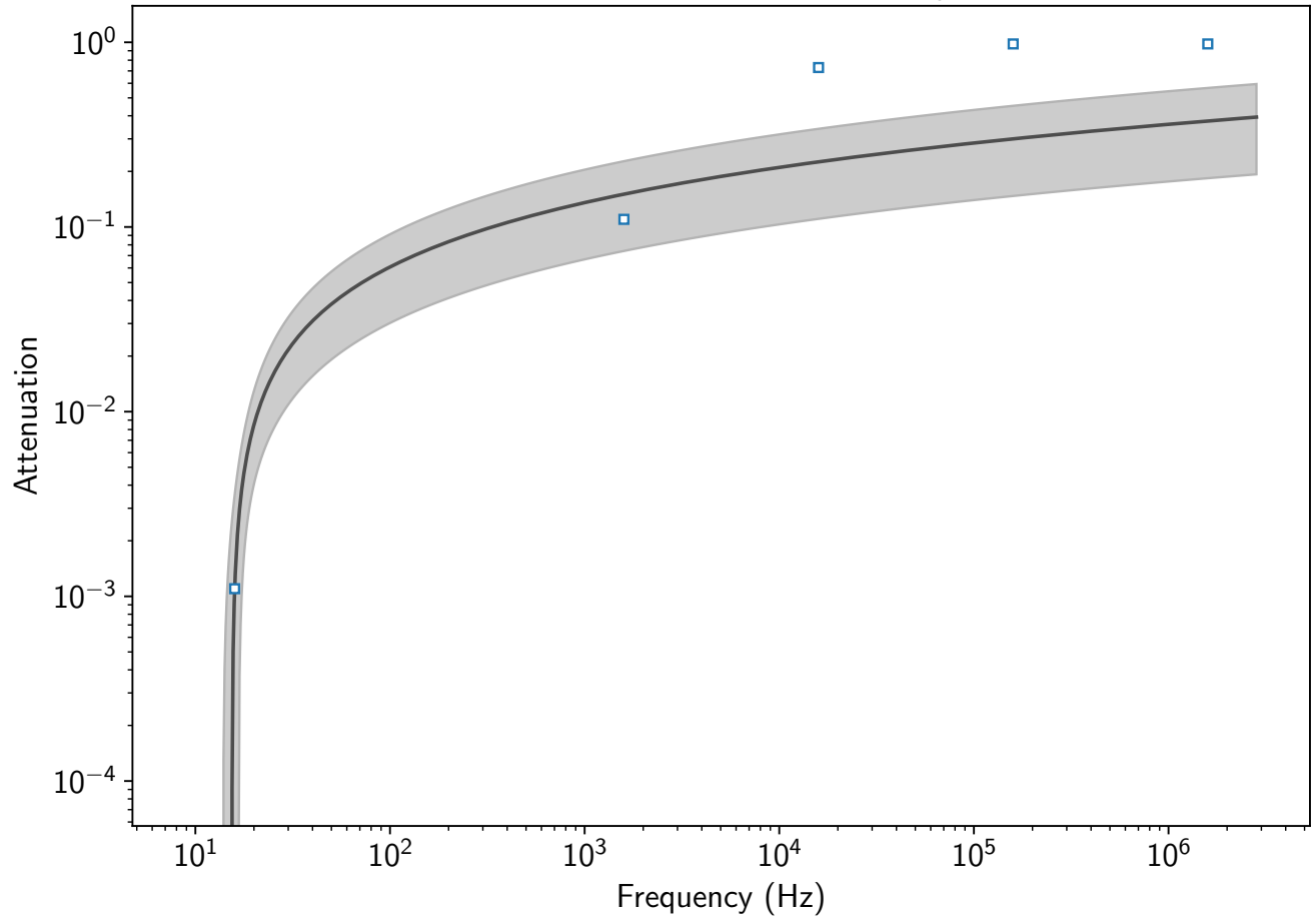
Attenuation vs Frequency
