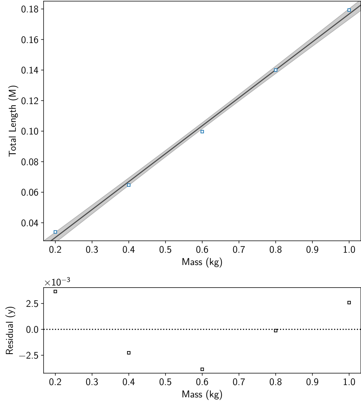
A graph that details the length of a spring when masses are hung on it
