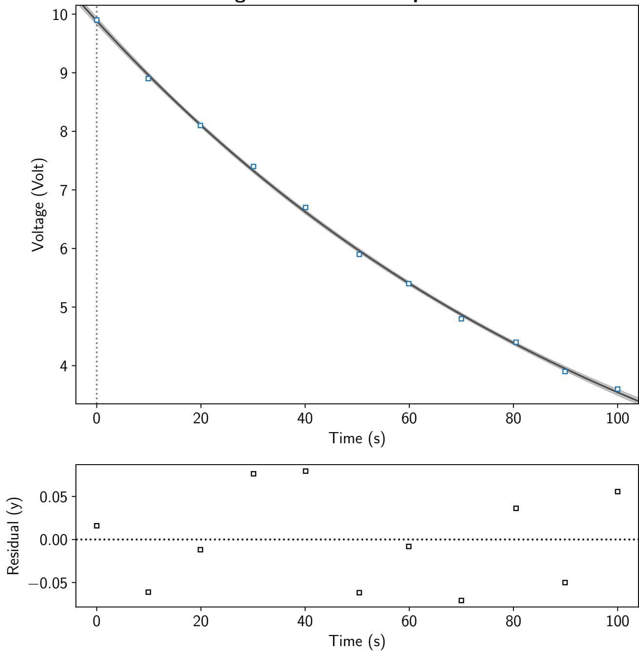
Voltage versus Time - Exponential Fit
