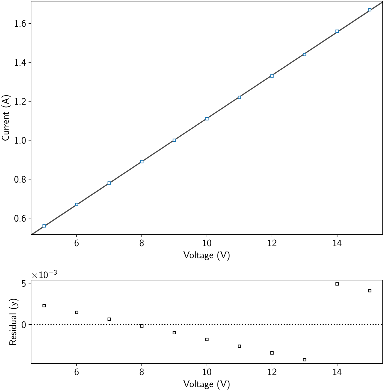
Voltage vs. Current of a circuit system
