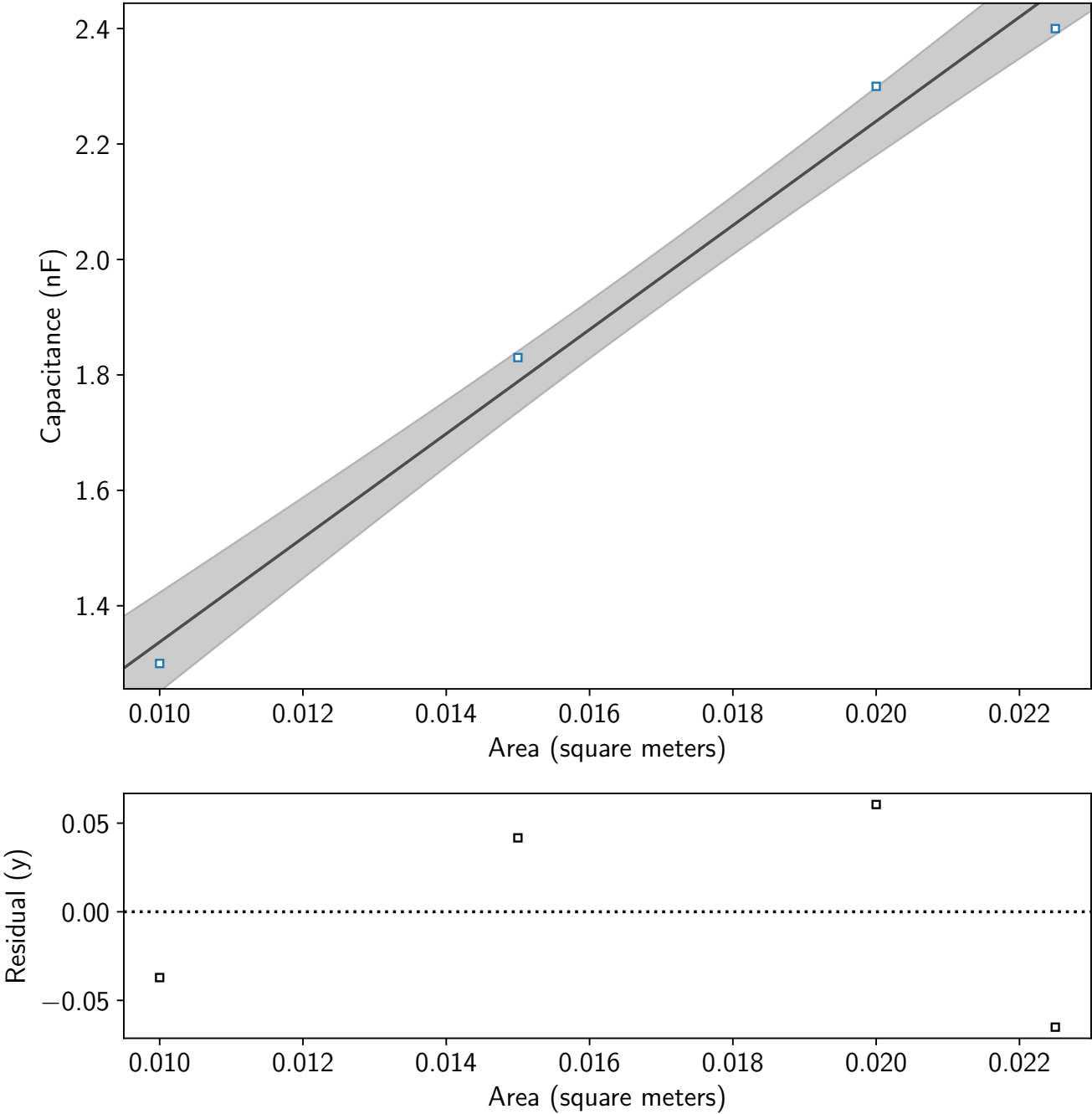
Capacitance versus area graph
