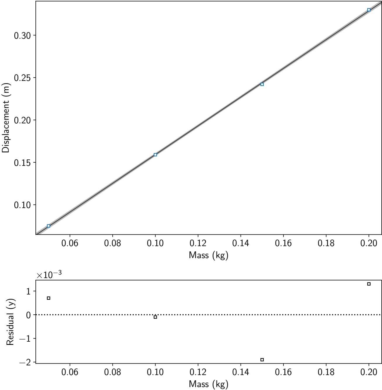
Static Measurement of Spring Constant
