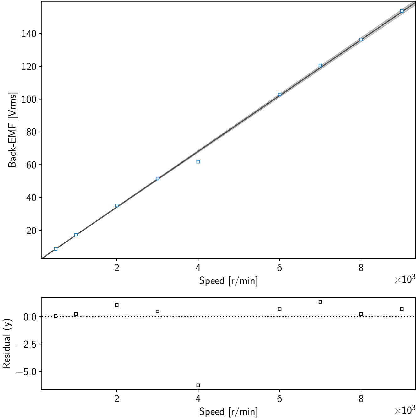
Back-EMF versus Speed
