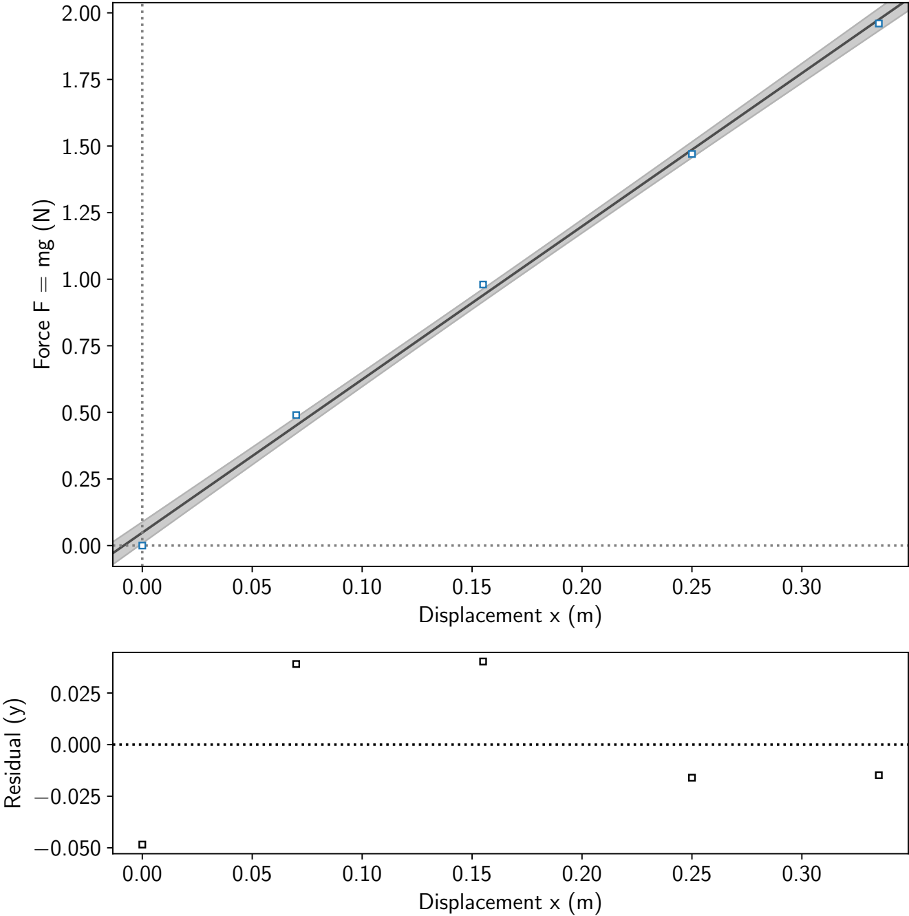
Spring Force vs Displacement
