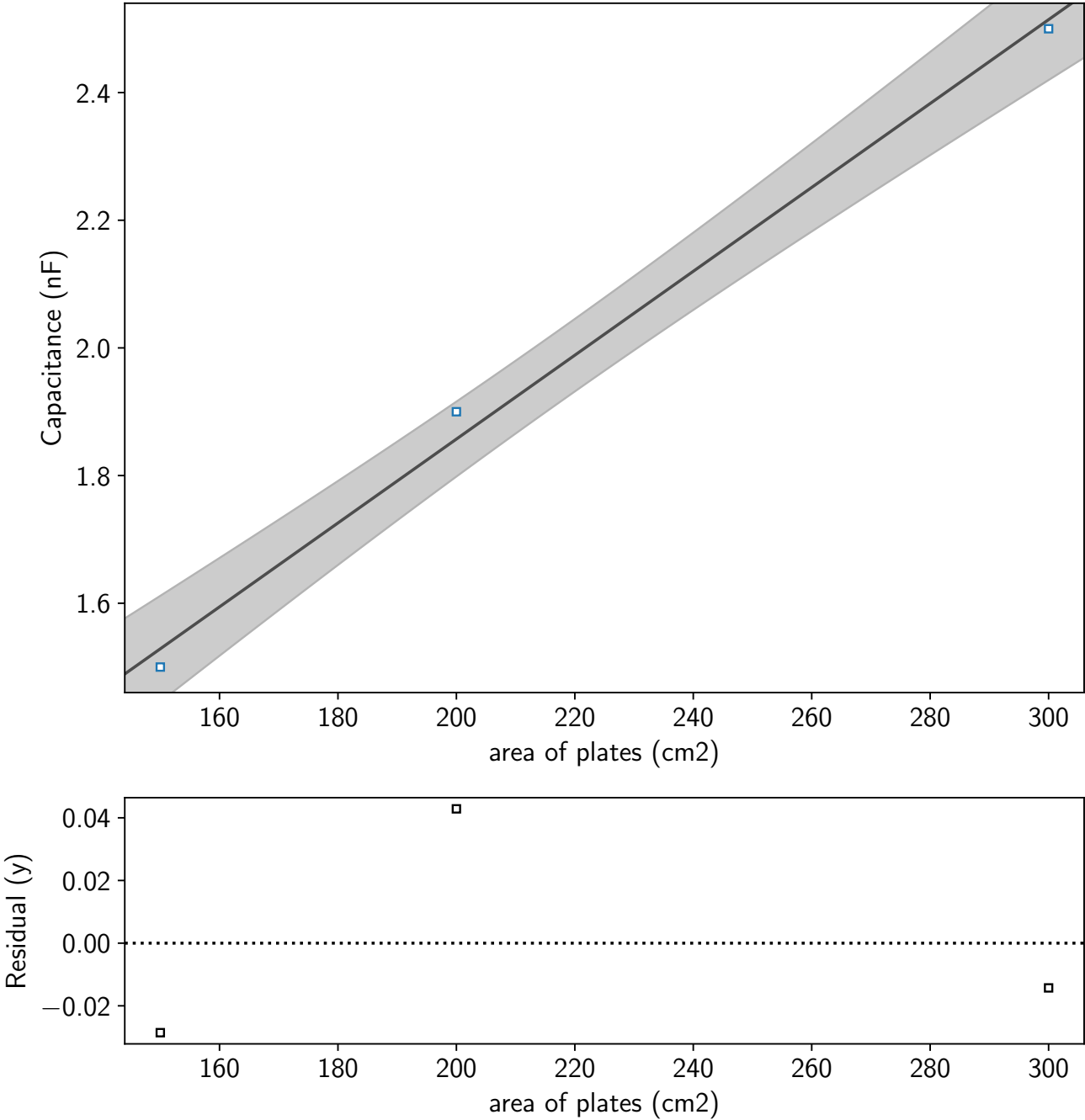
Capacitance vs Area of plates
