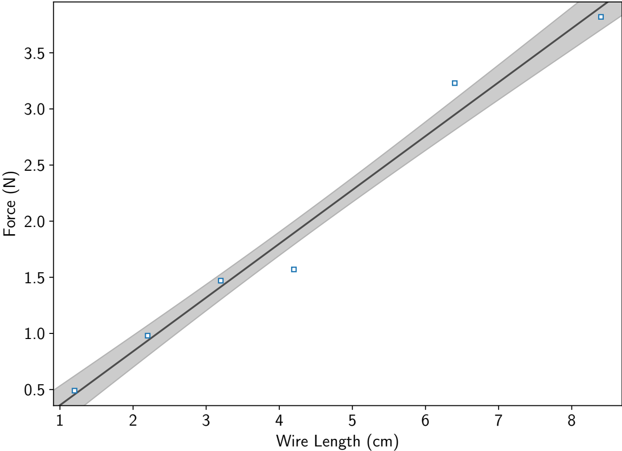
Force vs. Wire Length at Constant Current and Magnetic Field
