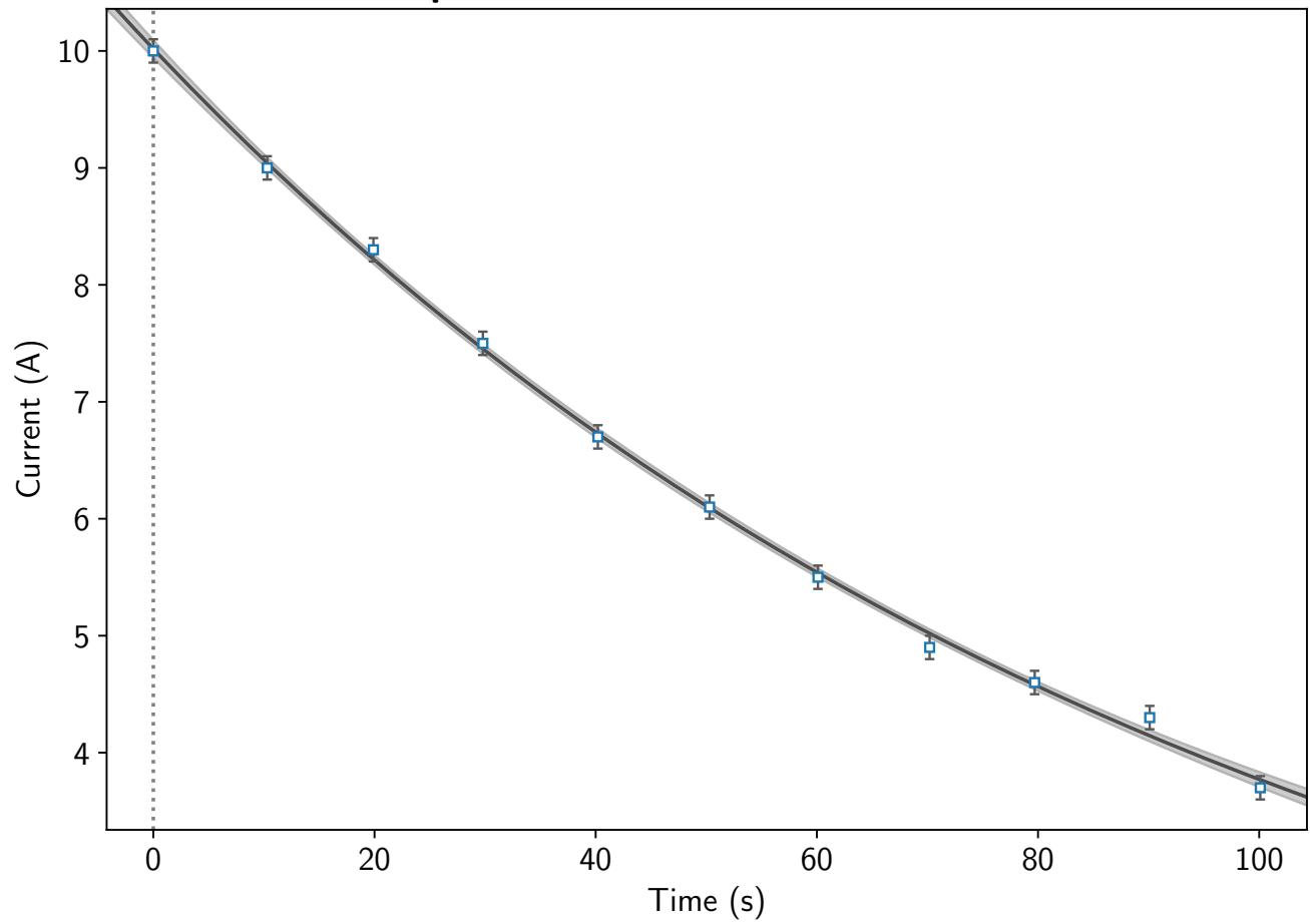
Exponential Fit of Current vs Time
