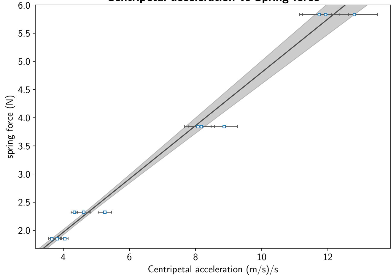
Centripetal acceleration vs Spring force
