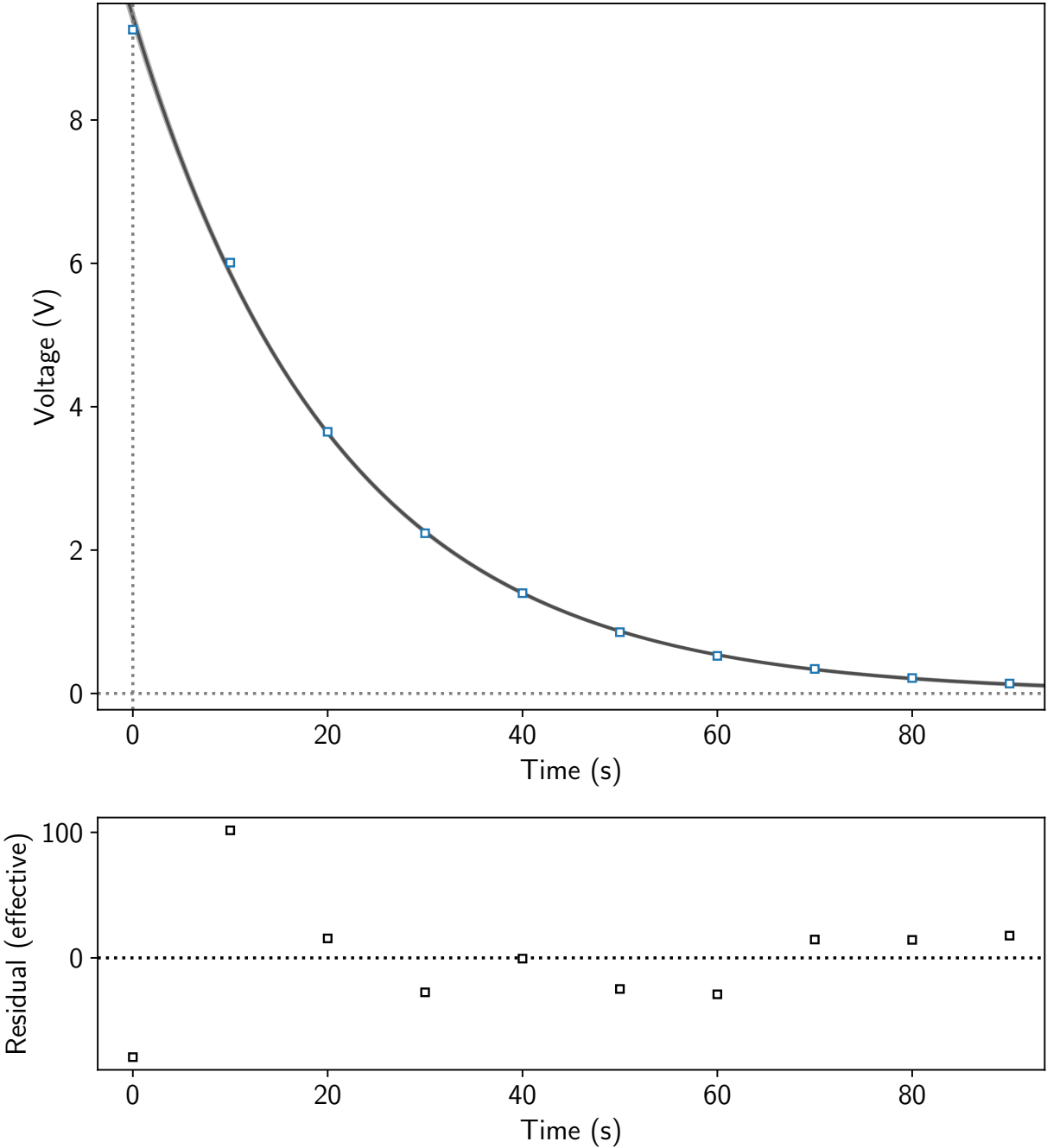
Relation between the time (s) and charge measured by voltmeter (V)
