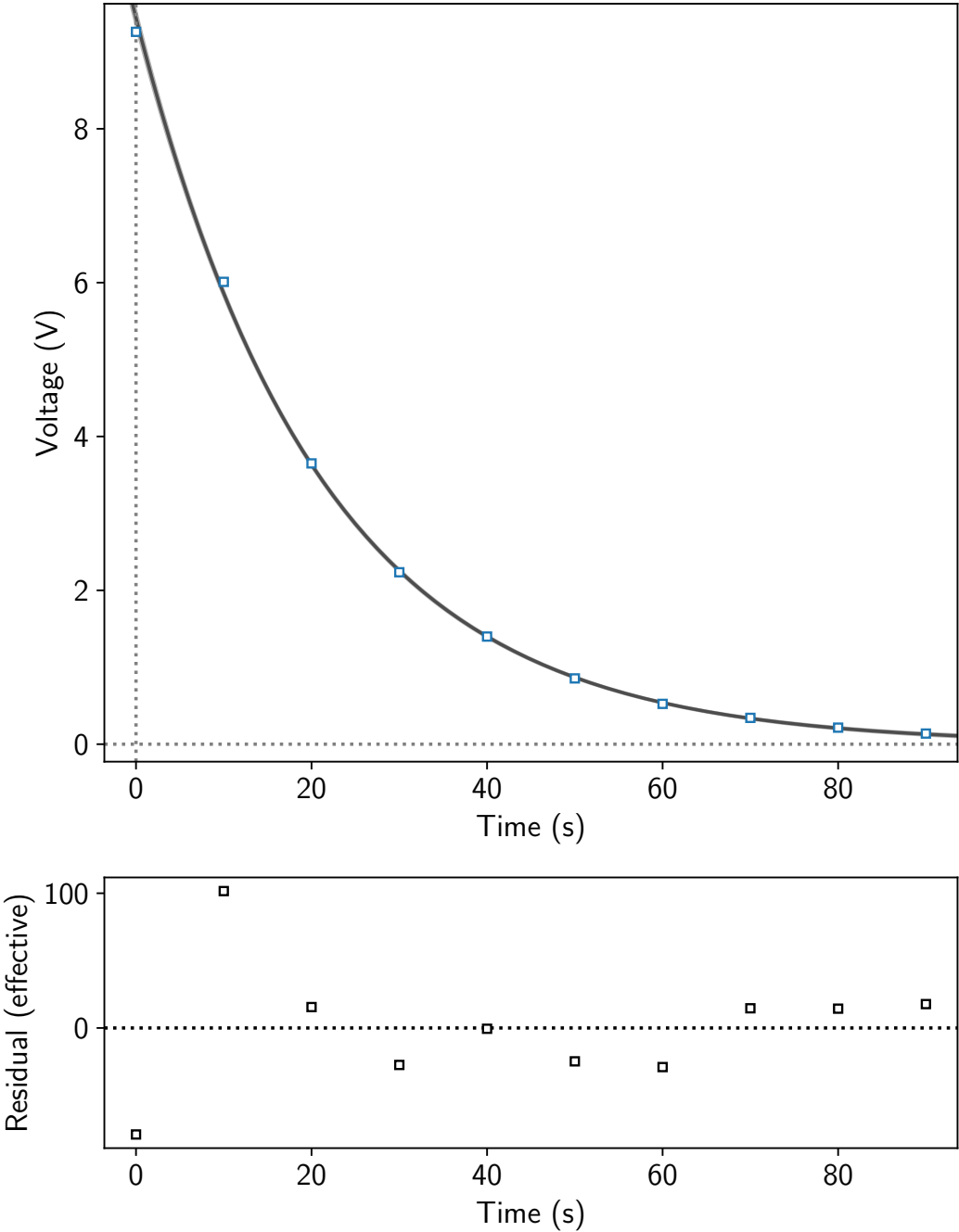
Relation between the time (s) and the charge decay measured by voltmeter (V)
