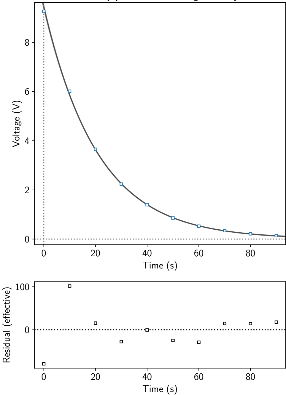
relation between the time (s) and the charge decay measured by voltmeter
