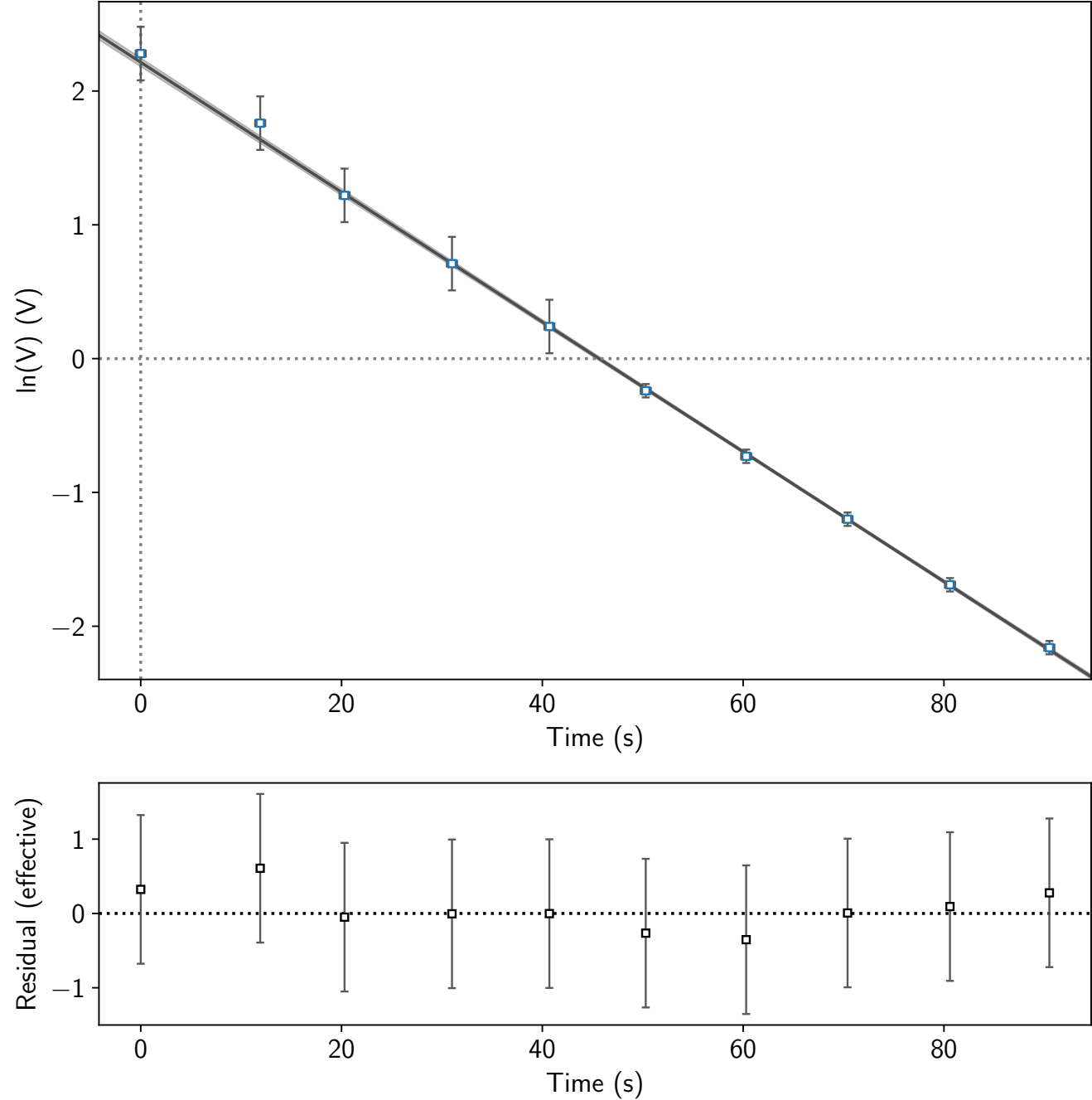
Discharge of the Capacitor: ln(V) (V) vs Time (s)
