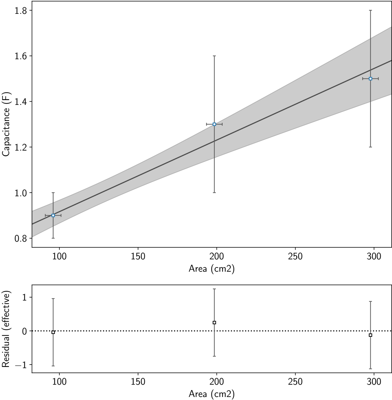
Capacitance as a function of area
