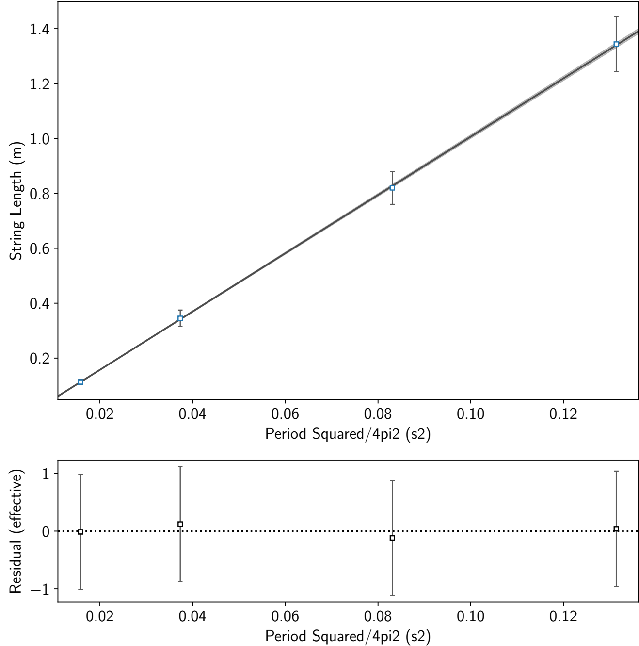
Pendulum Experiment
