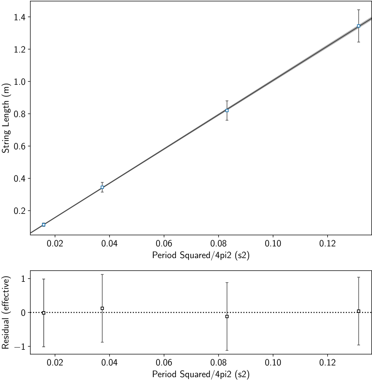
Pendulum Experiment
