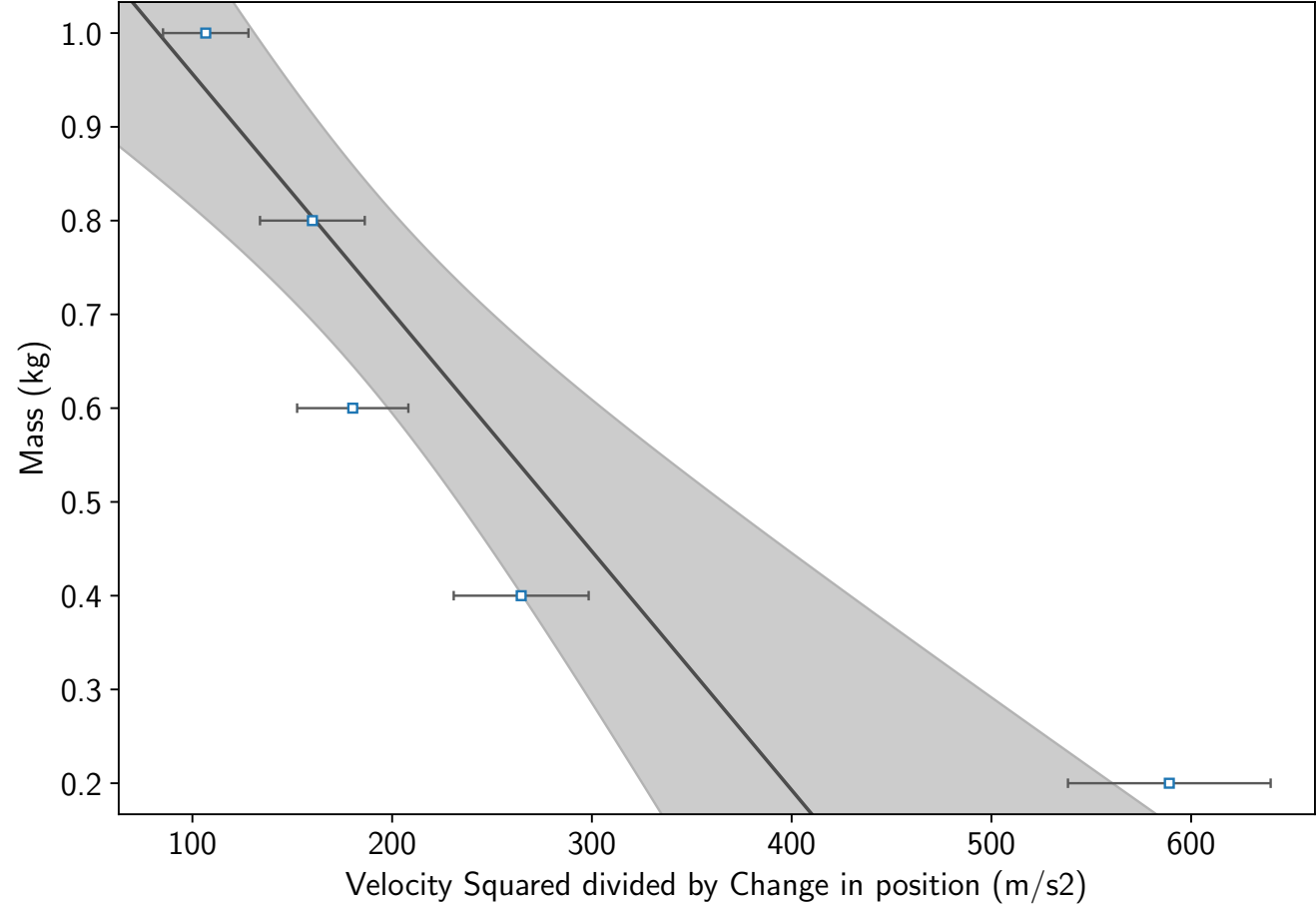
Force on ball by piston (HW Problem 1)
