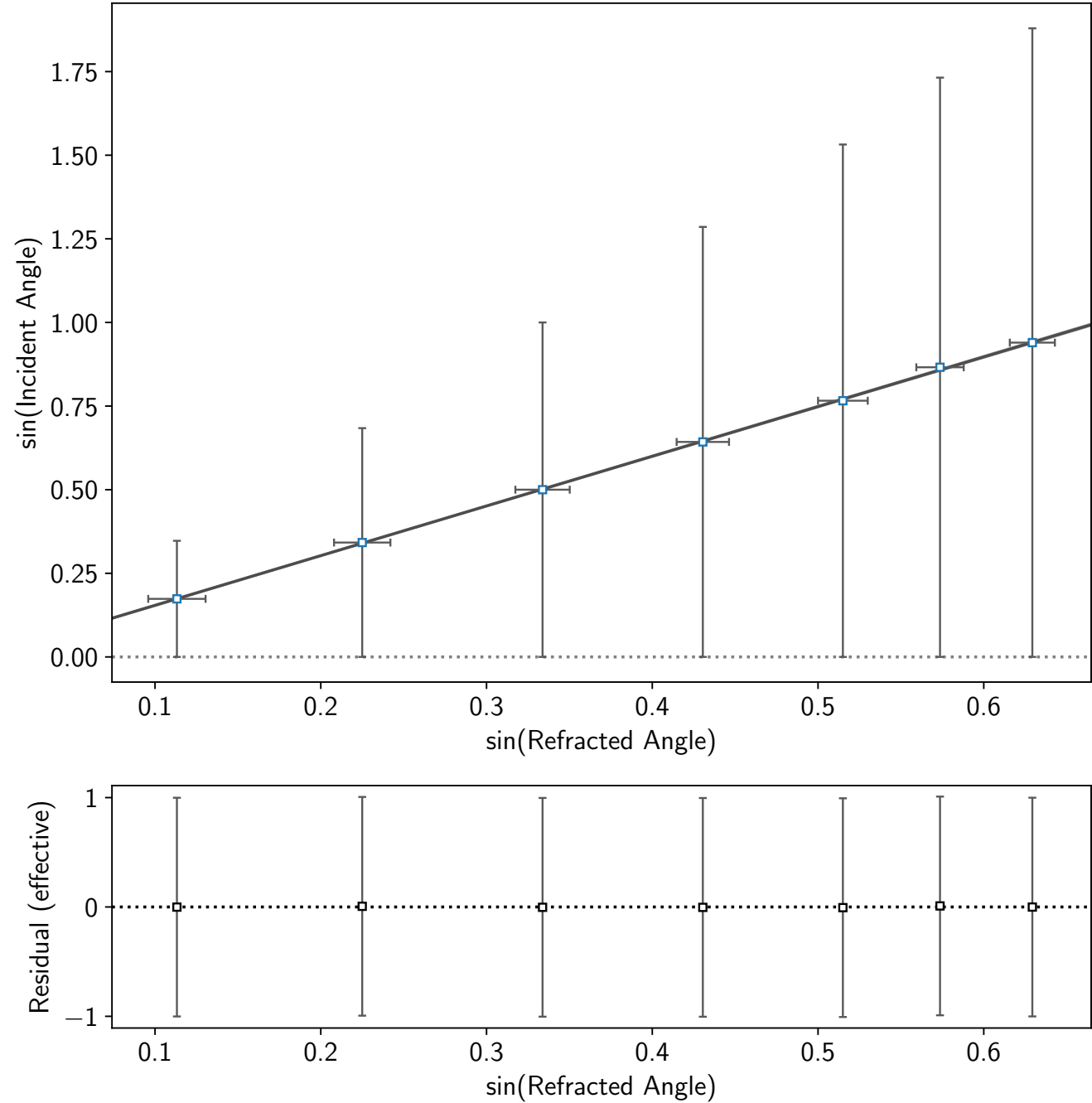
Sine of Incident Angle vs. Sine of Refracted Angle
