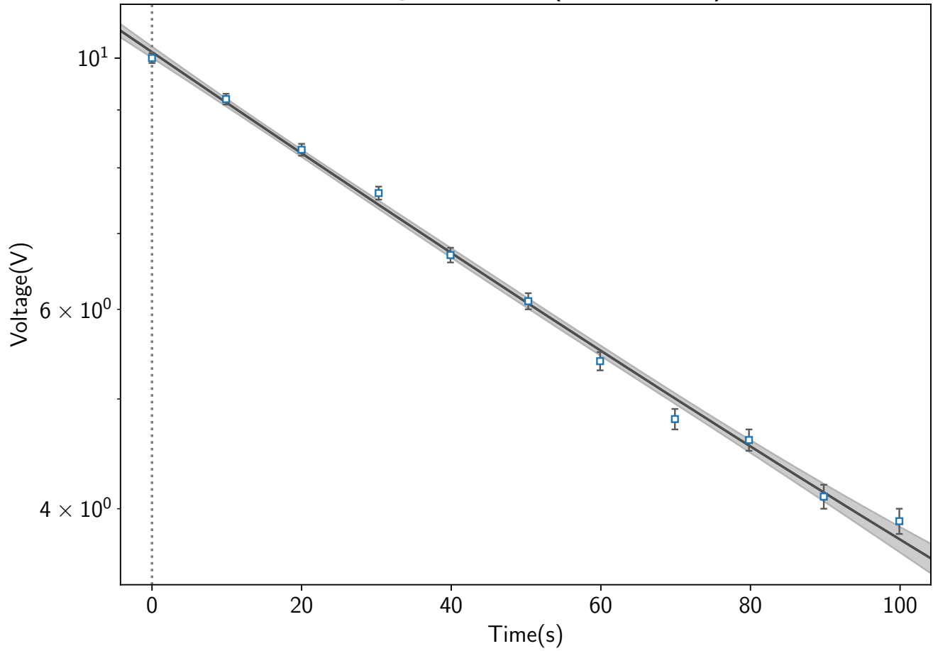
Voltage vs. Time(Exponential)
