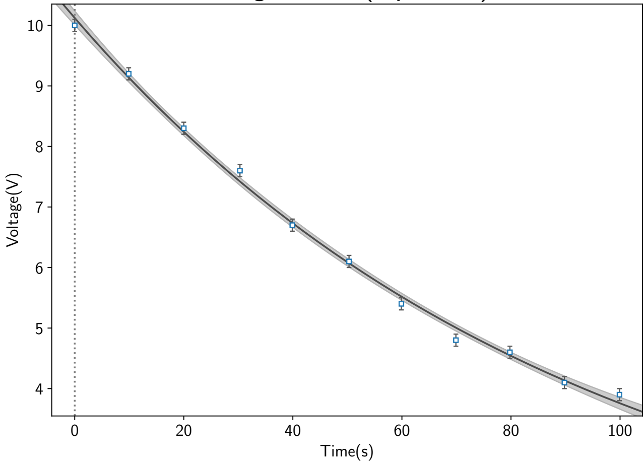
Voltage vs. Time(Exponential)
