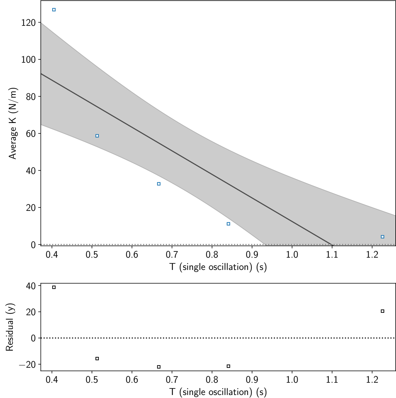
T (single oscillation) (s) vs. k (N/m)
