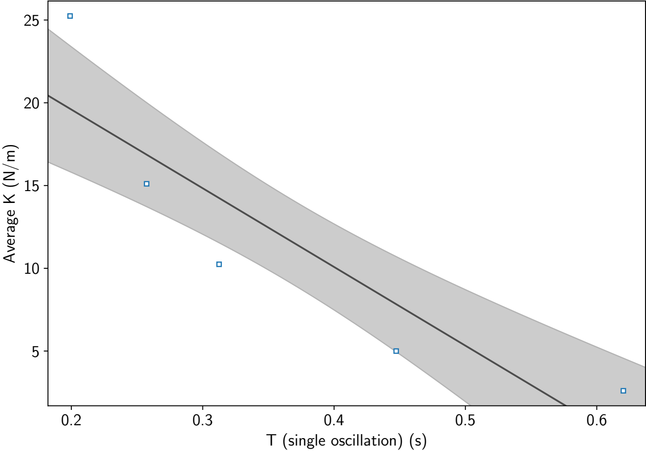
T (single oscillation) (s) vs. k (N/m)
