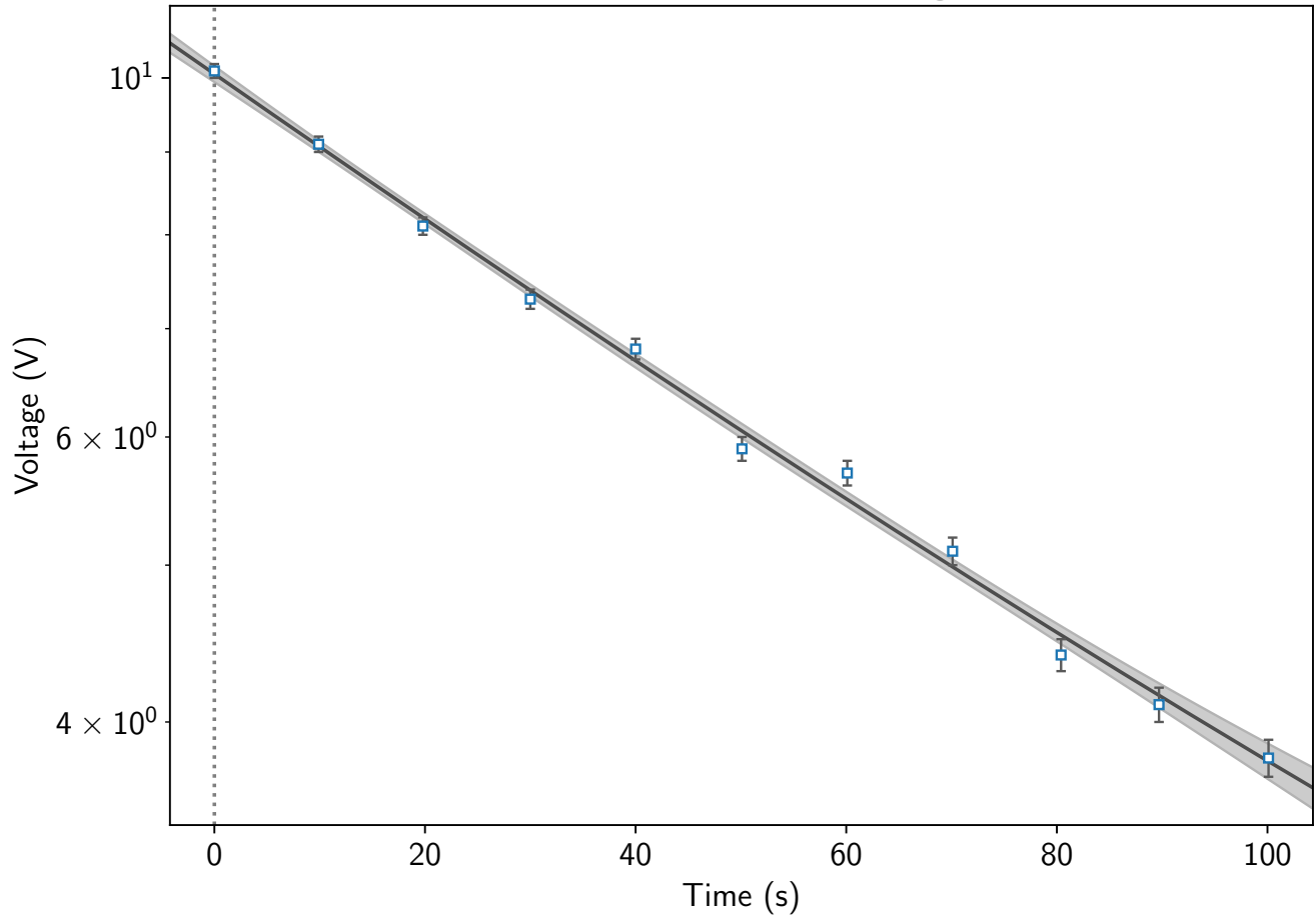
Exponential Fit: Capacitor Voltage vs. Time
