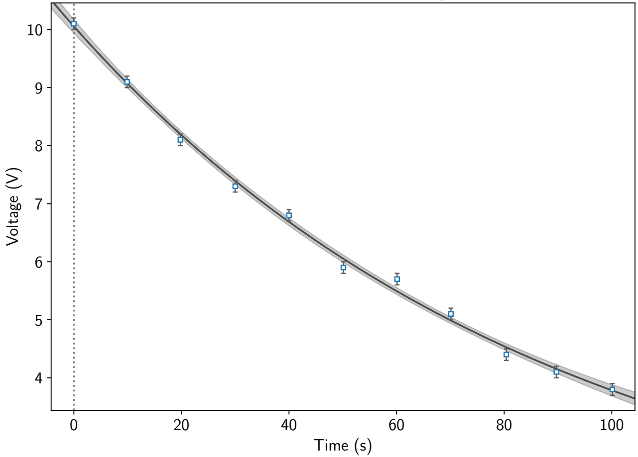
Exponential Fit: Capacitor Voltage vs. Time
