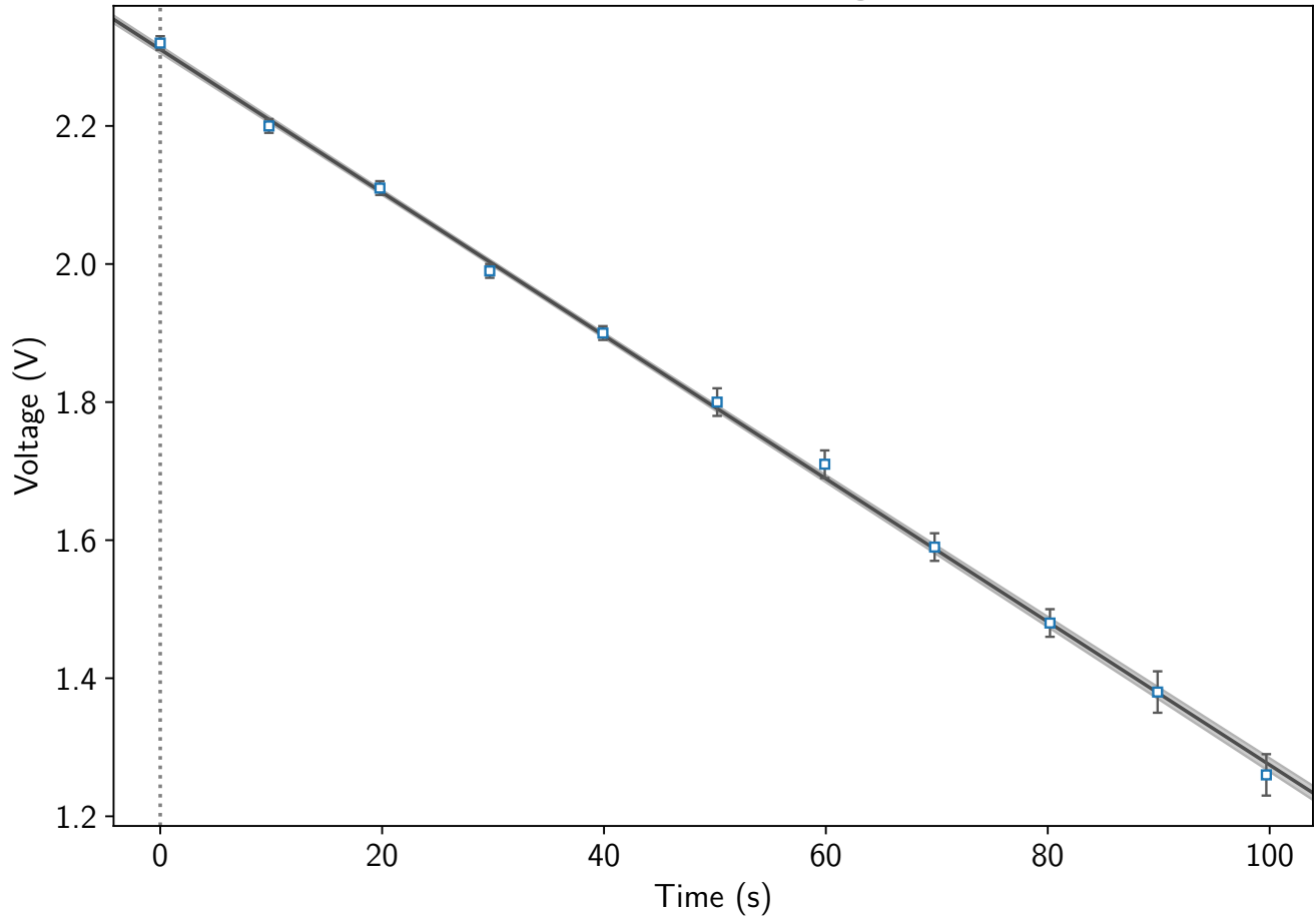
Linear Fit: Capacitor Voltage vs. Time
