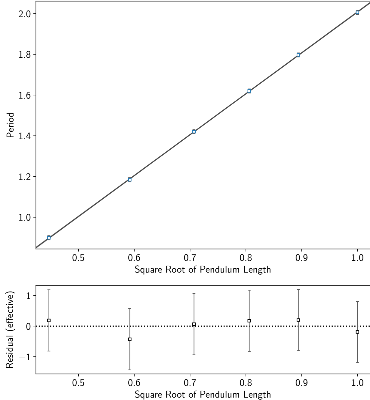
Relationship Between Period and Square Root of Pendulum Length
