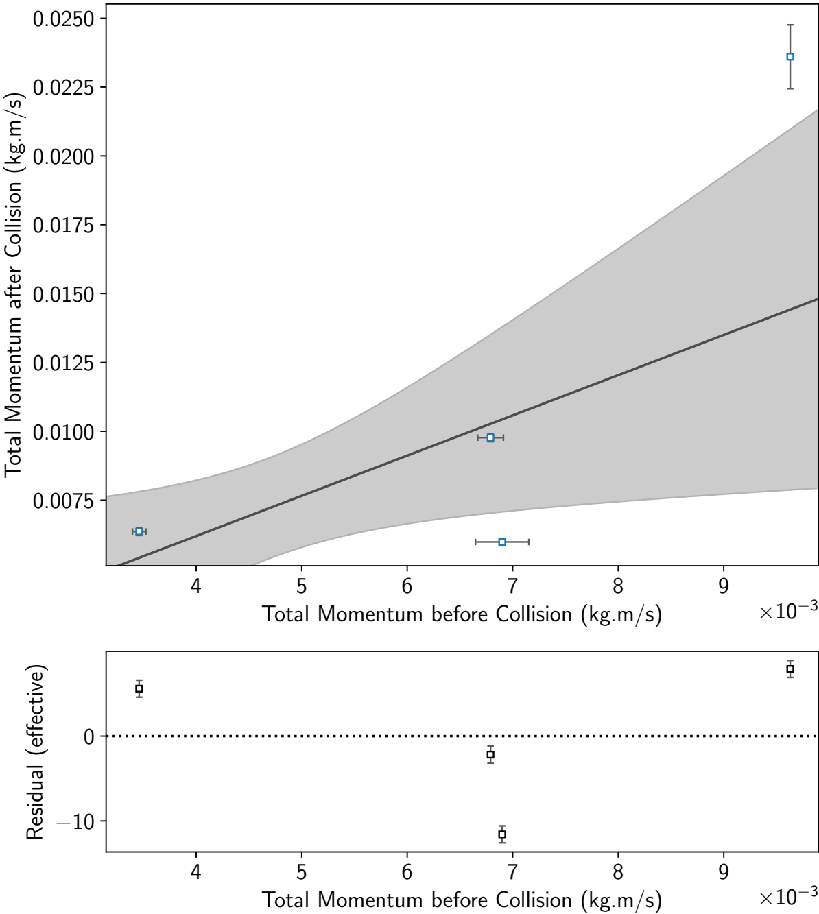
Total Momentum before Collision vs. Total Momentum after Collision
