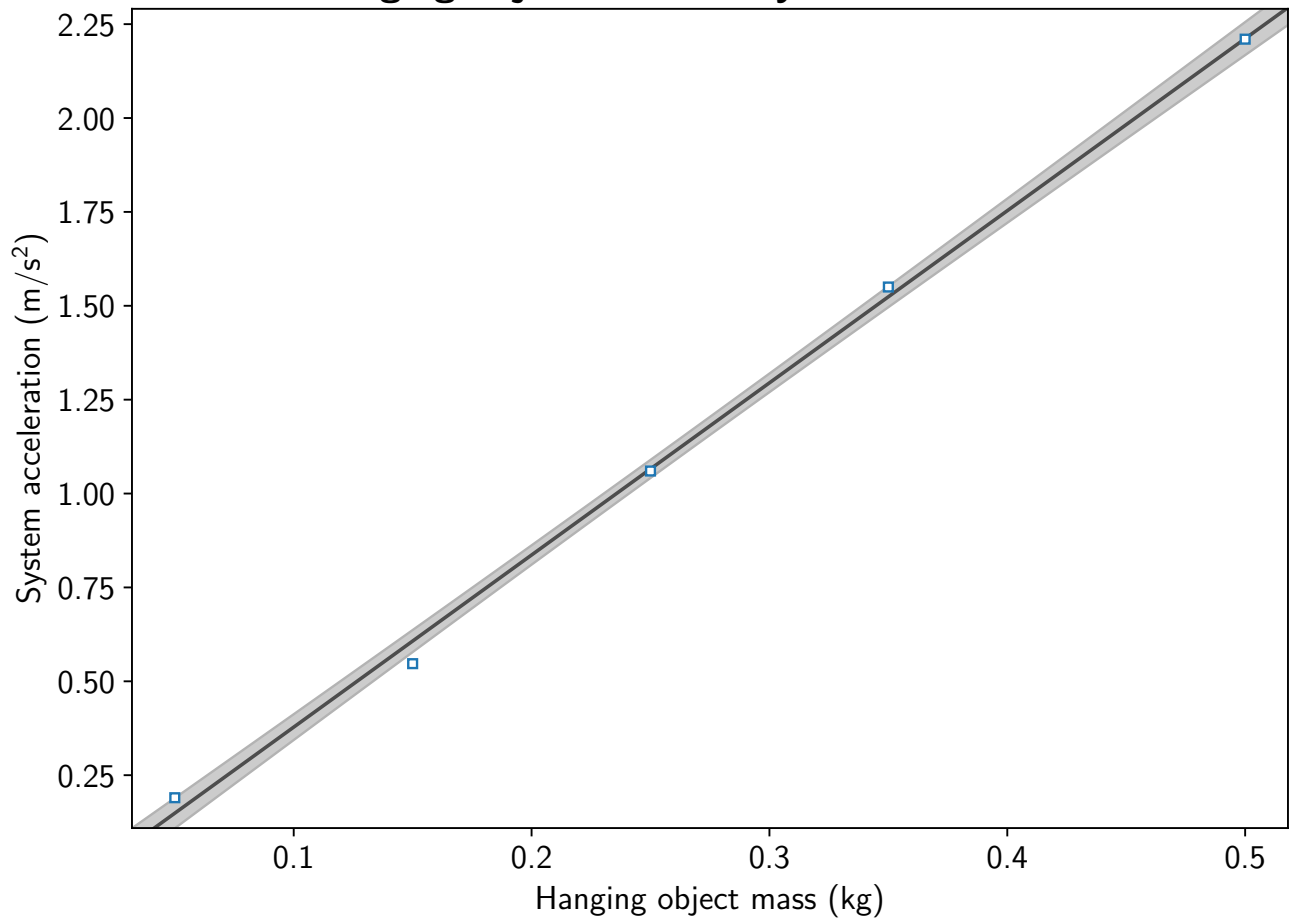
Hanging object mass vs System acceleration
